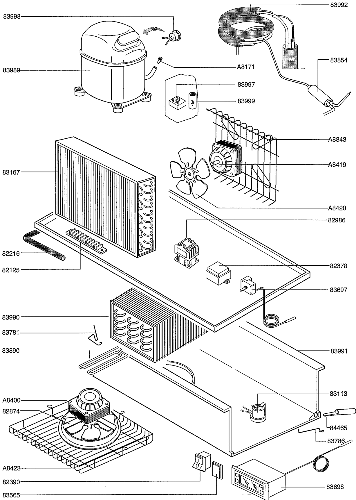
cooling unit assembly : A9294
